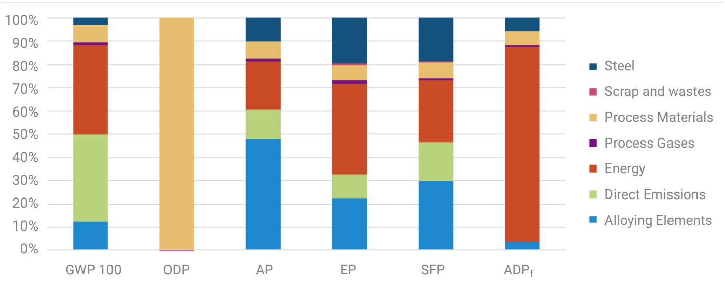
Figure 2: Relative results by category, wire rod
